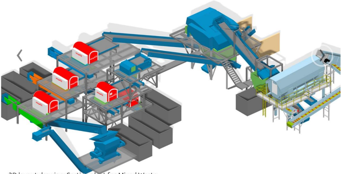
3D layout drawing: Sorting plant for Mixed Waste
